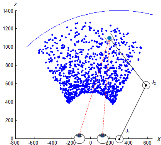
Fig. 4. Gazing and reaching schema. At each training step the artificial agent, either model or robot, is required to move its hand and gaze toward the same point, and update its sensorimotor representation using the observed error.
