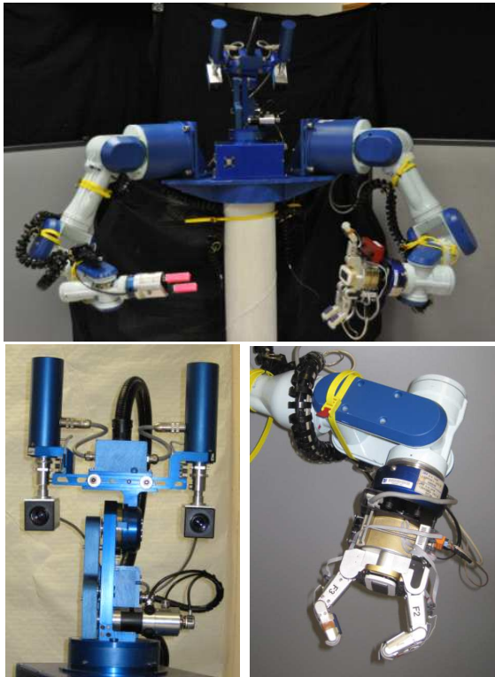
Fig. 8. Humanoid robot with detail of pan/tilt/vergence head and arm with hand.
