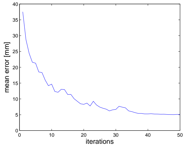
Fig. 7. Typical learning curve to adapt to the new parameters after the kinematics of the robot model has been changed.
