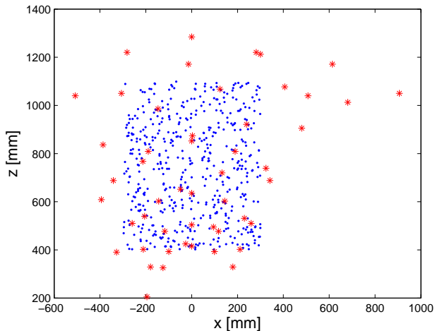
Fig. 6. Radial basis functions distributed according to a mixed (25 oculomotor + 25 arm motor) criterion (red stars), visualized over a typical Cartesian training set (blue dots).
