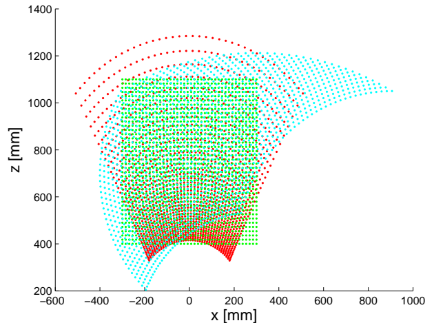
Fig. 5. Mapping of the space according to uniform distributions in a vergence/version oculomotor space (red), in a J1/J2 joint space (cyan) and in a standard Cartesian space (green).
